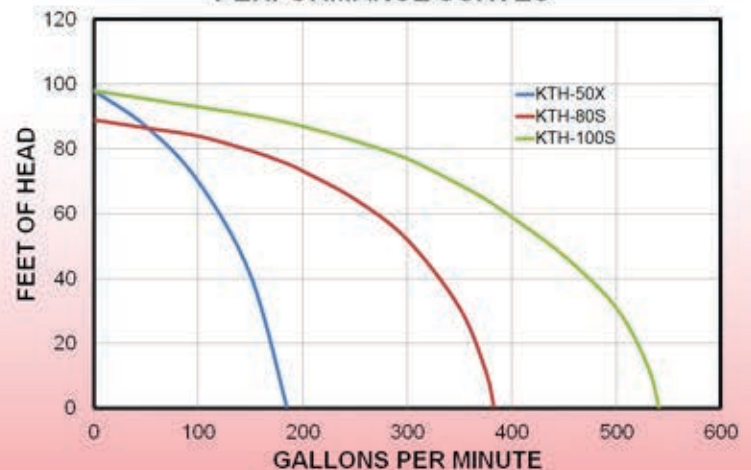
PERFORMANCE CURVES
