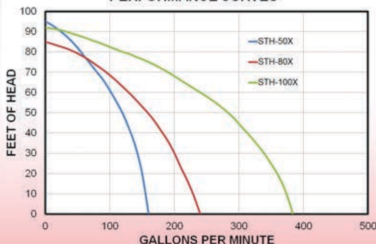
PERFORMANCE CURVES
