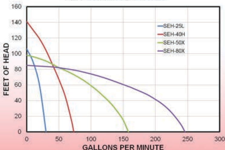
PERFORMANCE CURVES
