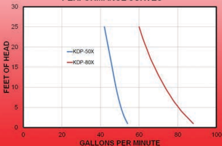
PERFORMANCE CURVES
