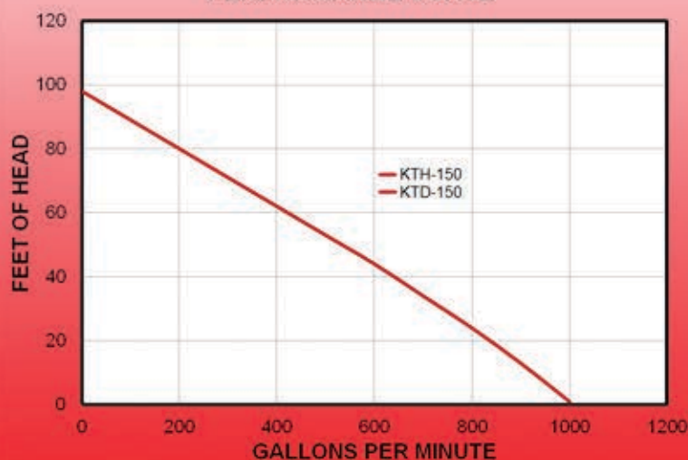
PERFORMANCE CURVE
