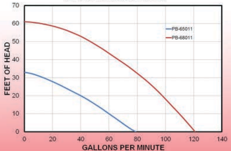
PERFORMANCE CURVES
