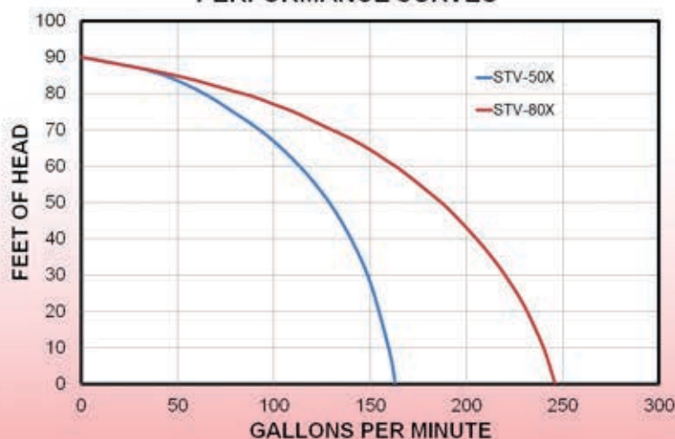
PERFORMANCE CURVES
