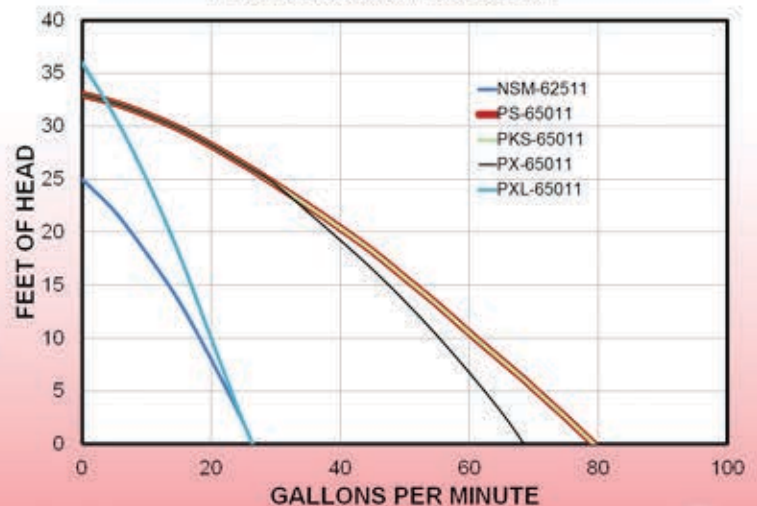
PERFORMANCE CURVES
